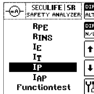
Selecting current of applied parts – direct/equivalent leakage current measurement – polarity reversal
