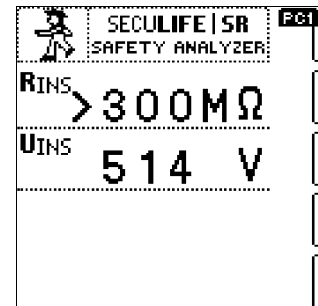
Display of insulation measurement – Display of protection class
