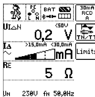
Earthing Resistance Meas. Display
